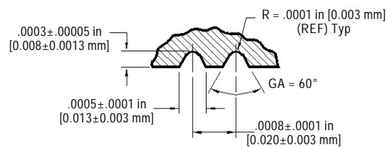
TYPICAL GROOVE DETAIL
