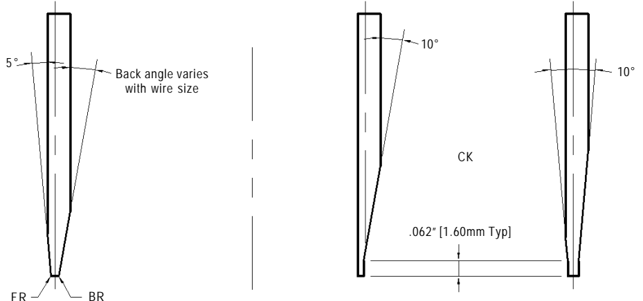
Shank Style A (Standard)
