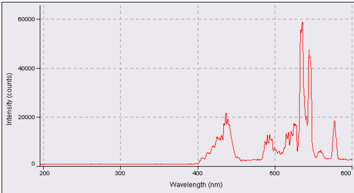
UV BLOCKING RIGID FILTER, CLEAR – ITEMS: F007-002, 002C, 002CLR
