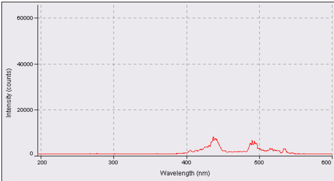
UV BLOCKING RIGID FILTER, BLUE – ITEMS: F007-022, 022B
